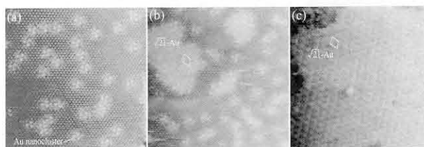
Figure 1 Topographic STM images of Au-adsorbed \sqrt{3} -Ag surface taken at 65 K and at various Au coverages: (a) 0.016 ML, V_{tip} = -0.50 V, I = 0.75 nA; (b) 0.048 ML, V_{tip} = -0.50 V, I = 0.75 nA; (c) 0.136 ML, V_{tip} = -1.50 V, I = 0.50 nA. The size of each image is 31.2 \times 31.2 nm 2 .
