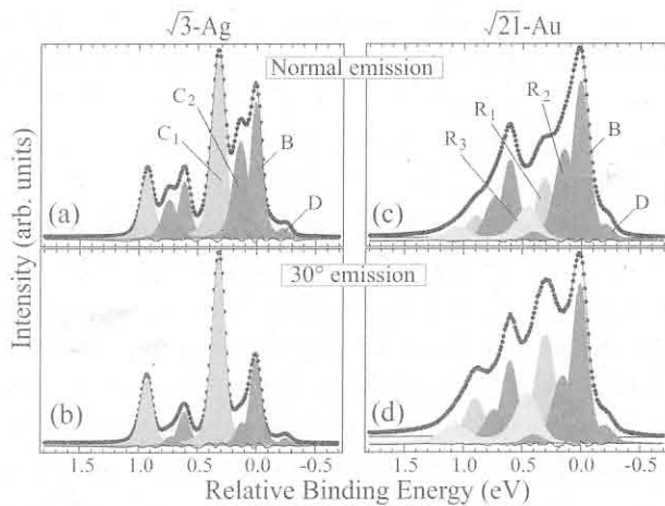
Figure 3 Si 2p CLS taken from the \sqrt{3} -Ag [(a), (b)] and \sqrt{21} -Au [(c), (d)], recorded at 70 K with photon energy of 135 eV at normal [(a), (c)] and 30° [(b), (d)] emissions. The spectra were taken on the beam line of BL-1C at the Photon Factory.
